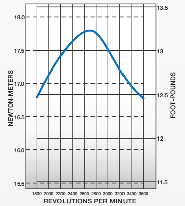
Net Torque
