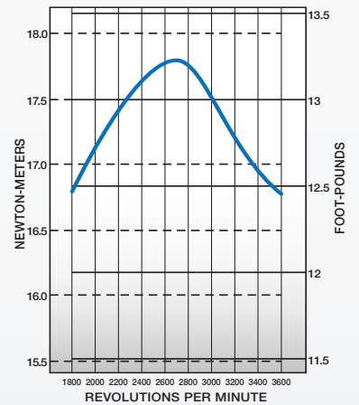
Net Torque
